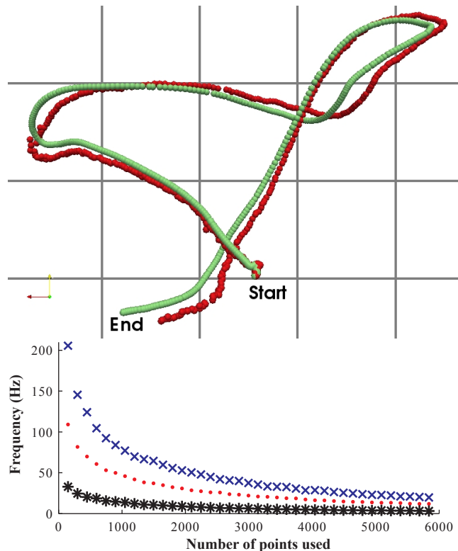
Figure 3 Tracking the pose of a Kinect RGB-D sensor in a home-like environment. Top : projection on the xy -plane of a tracked position (dark-red) versus the measured ground truth (light green). Each grid square is half a meter. Bottom : performance for different processors: Intel Core i7 Q820 (blue “x”), Intel Xeon L5335 (red “•”), and Intel Atom Z530 (black “*”).
